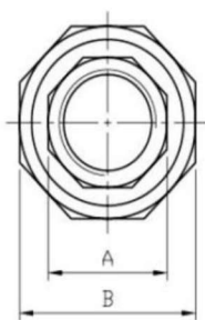
1/4" Hexagon 3/8"~2" Octagon 2-1/2"~4" Decagon
